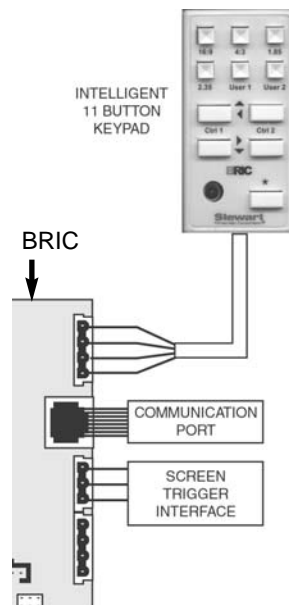
Figure 4. Connecting 11-button keypad to the BRIC
