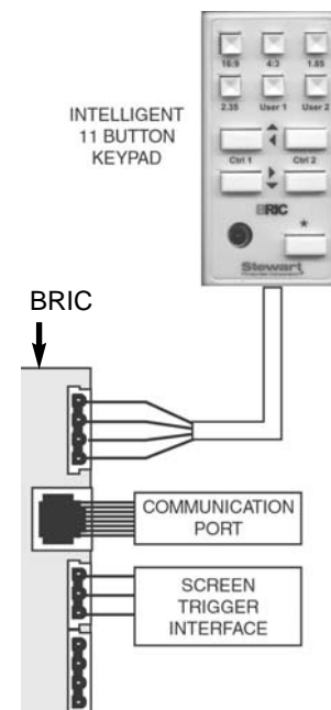
Figure 9. Connecting 11-button keypad to the BRIC
