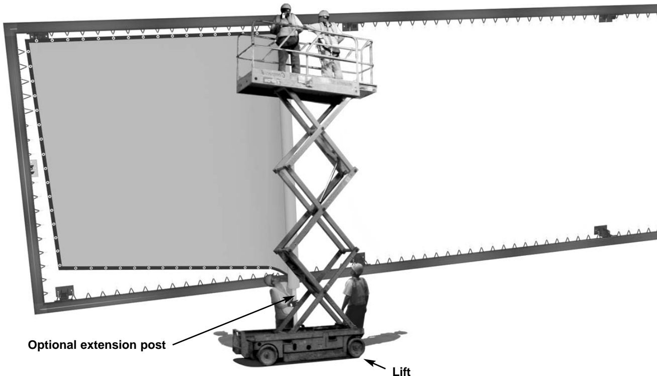
Figure 13. Beginning to attach screen to frame
