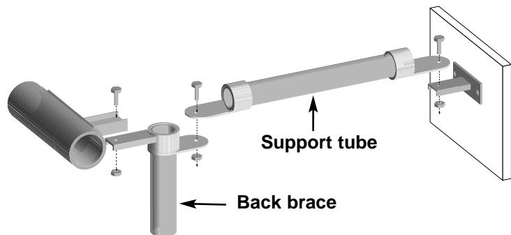
Figure 4. Wall mount for curved screen: Frame, back brace, support tube, wall bracket
