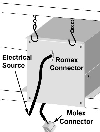
Figure 3: Electrical connection
