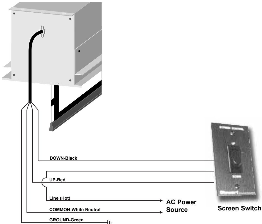
Figure 4: High voltage control wiring diagram
