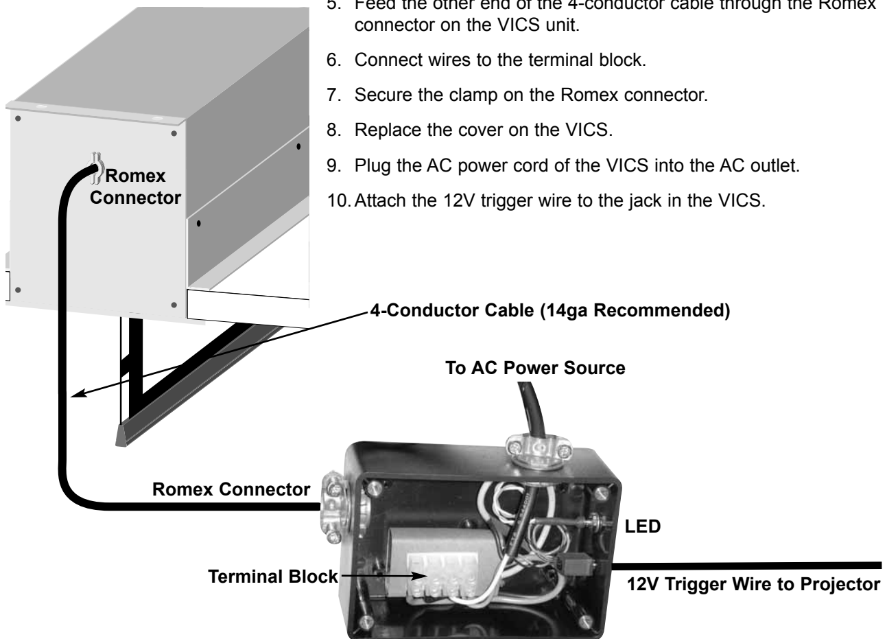
Figure 7: VICS connection
