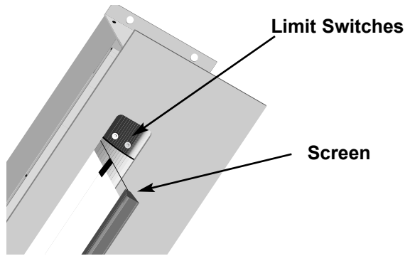
Figure 10: Underside view
