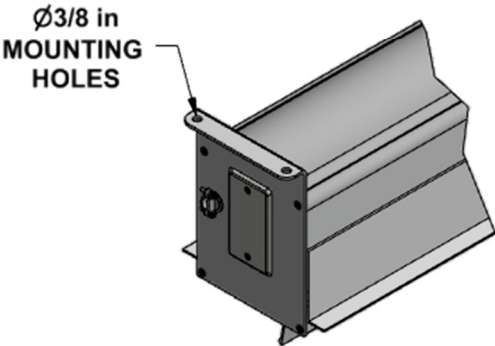
ISO DETAIL VIEW (NOT TO SCALE)
