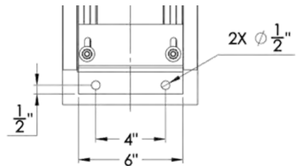
Figure 5. Ceiling Mount on top of Cascade unit
