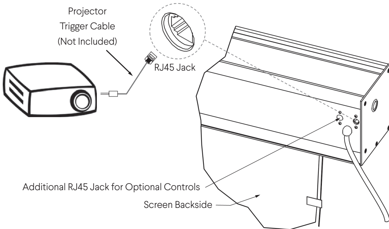
Figure 7: Projector Connection
