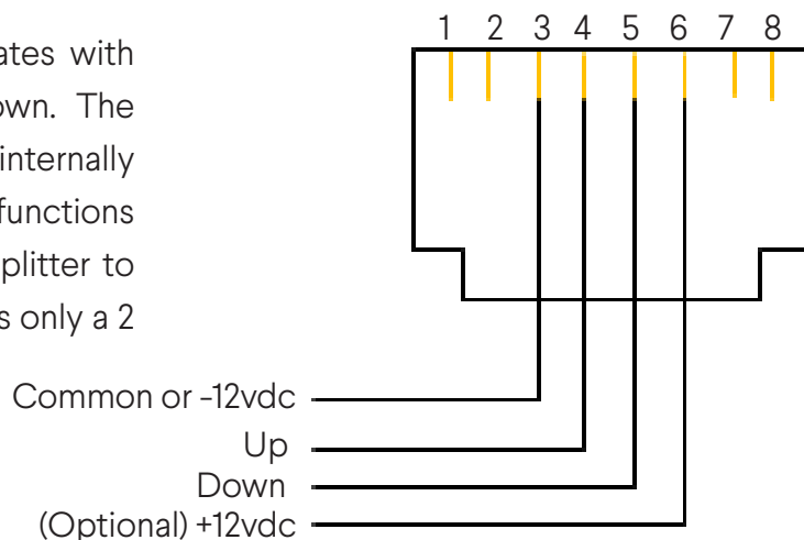
Figure 12: Pinout Diagram
