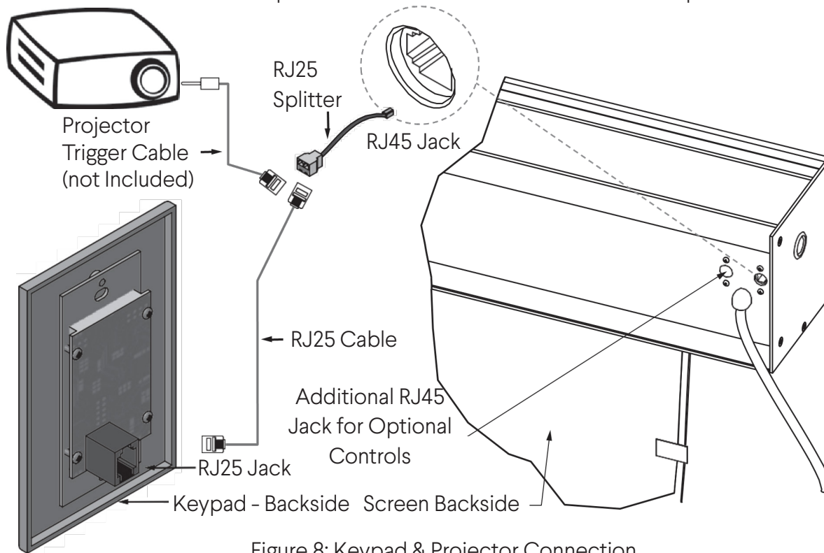
Figure 8: Keypad & Projector Connection
