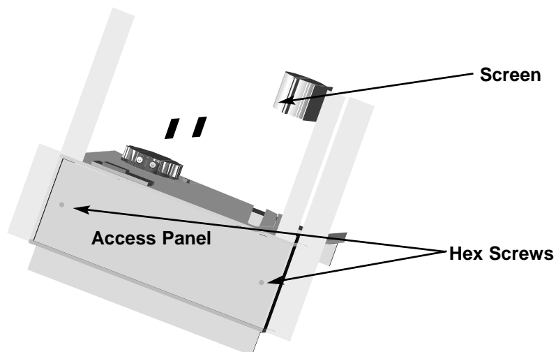
Figure 1: Stealth Grande underside view
