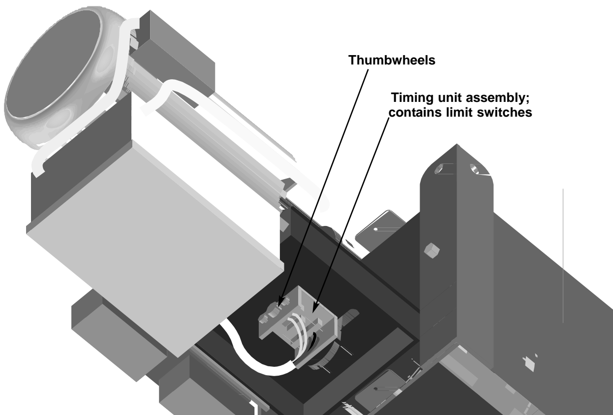
Figure 3: Underside view
