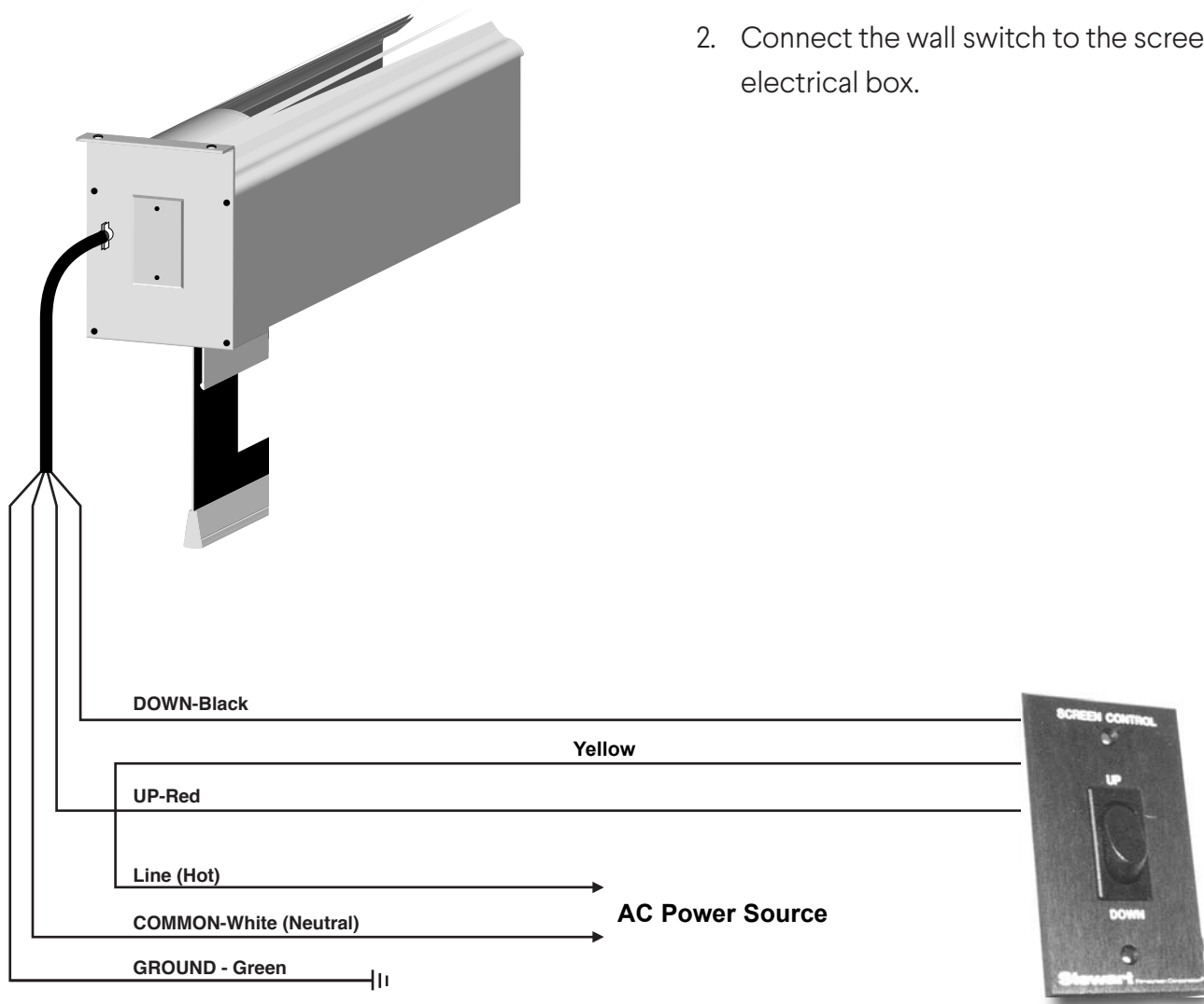
Figure 6: High voltage control wiring diagram
