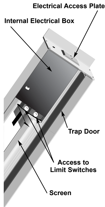
Figure 12: Underside view of Electriscreen
