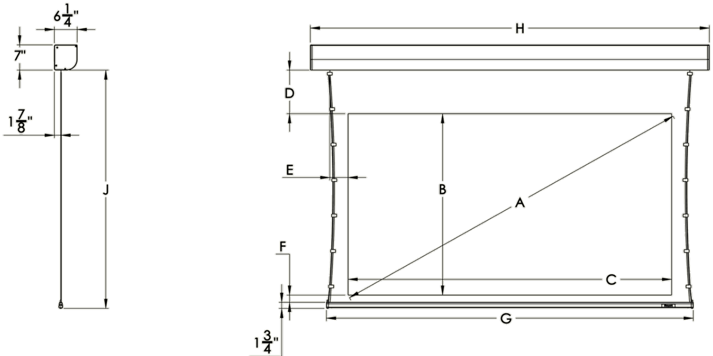
Figure 14: Basic front and side view drawing with letters for dimensions. See tables below for appropriate aspect ratio and dimensions.
