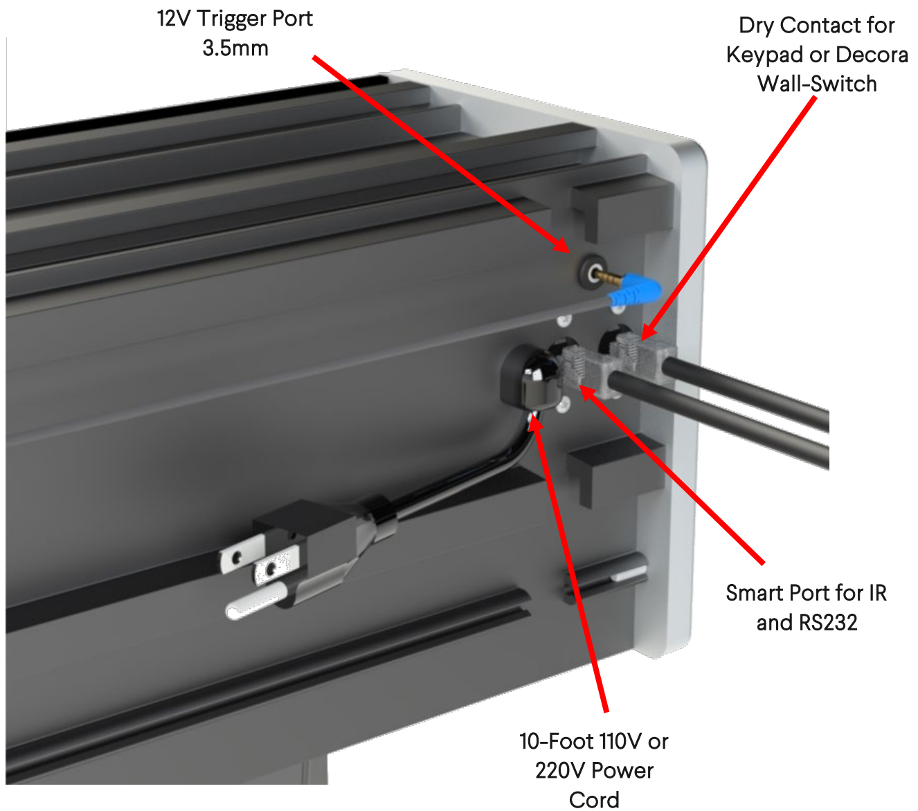
Figure 12: Back view, audience left hand side of Luxus G2 power control ports.
