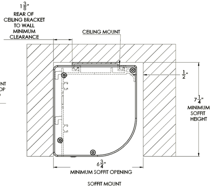
Figure 9: Conventional soffit mount configuration with minimum spacing dimensions for soffit.
