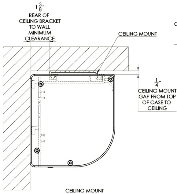
Figure 8: Conventional ceiling mount configuration with minimum spacing dimensions.
