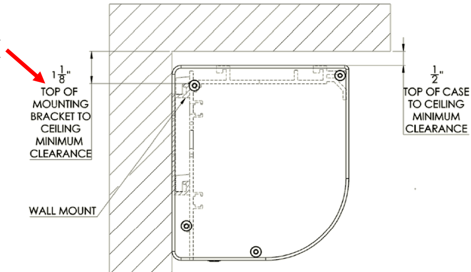
Figure 6: Drawing above shows the minimum dimensions that must be respected when installing Luxus G2 to the wall.
