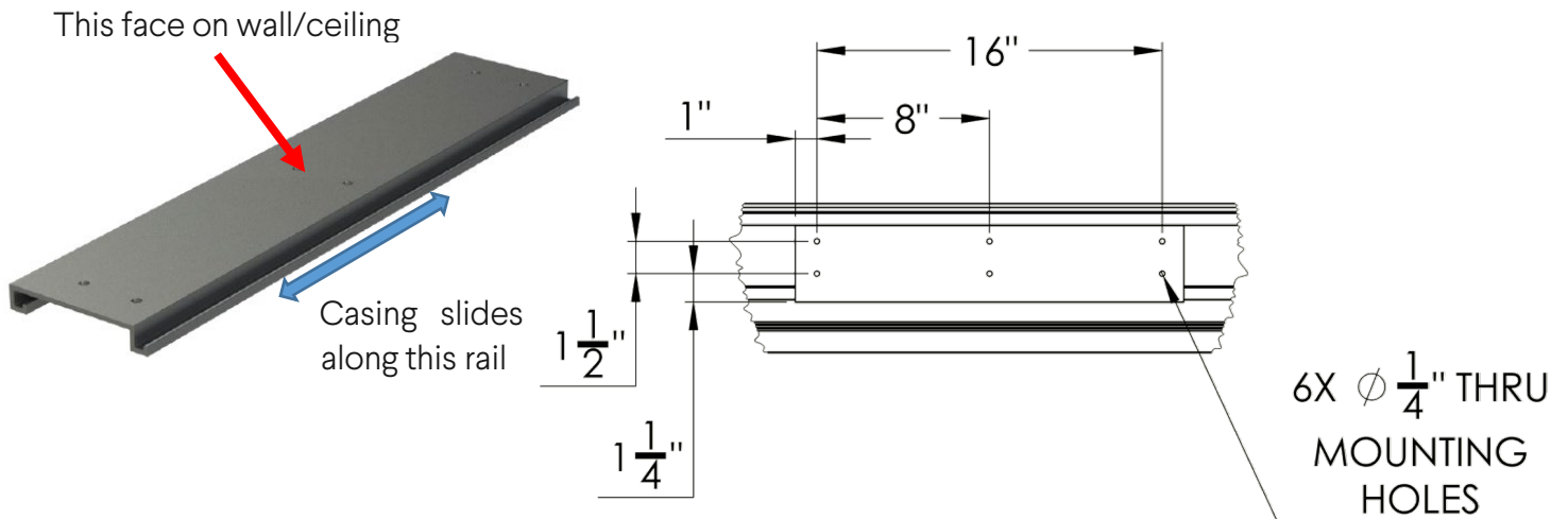
Figure 3: (From left) Isometric Render; Mount dimensions as viewed from mounting surface of mount.
