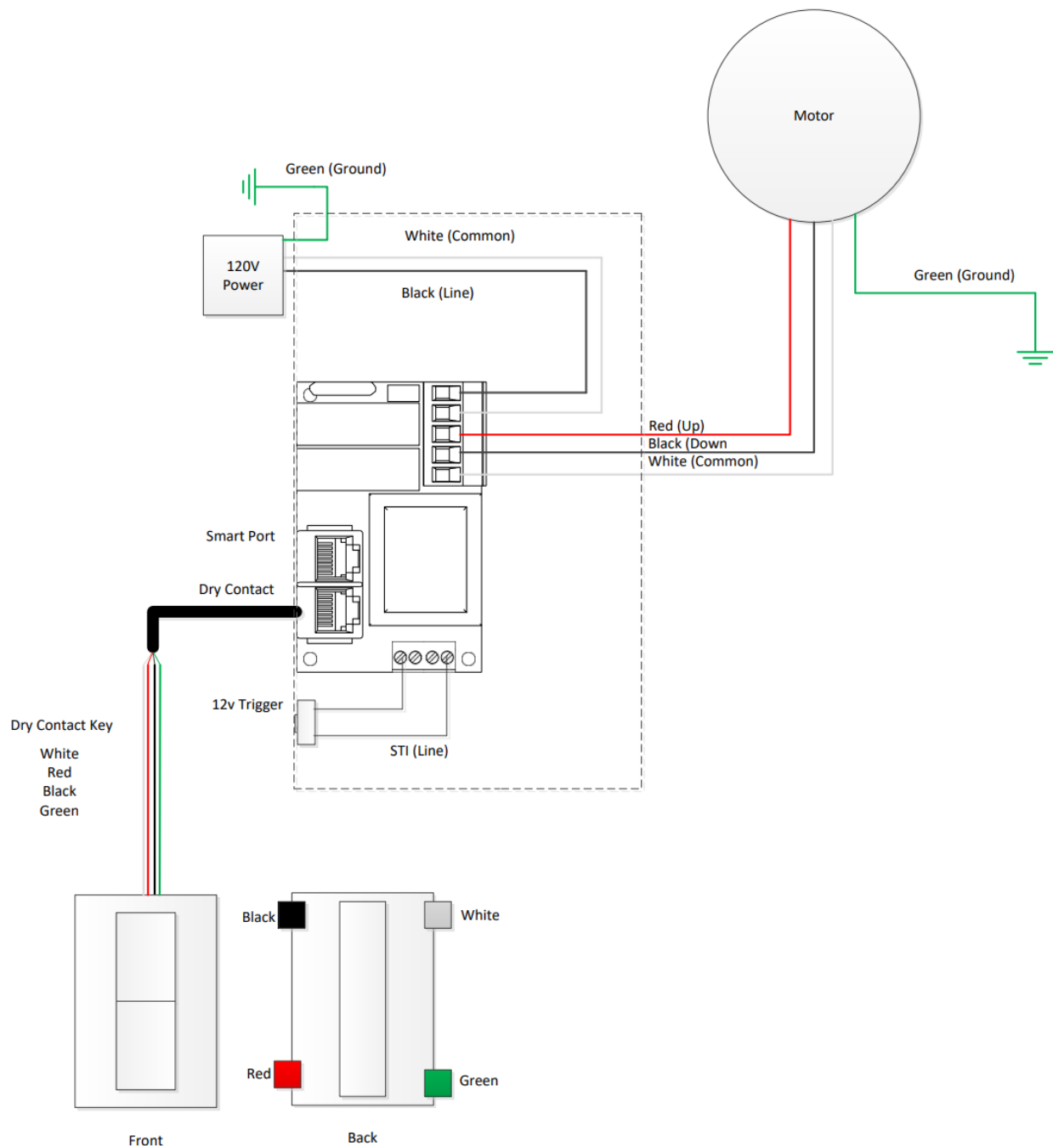
Figure 13: Luxus G2 internal wiring to IMC with standard color coded connections shown.
