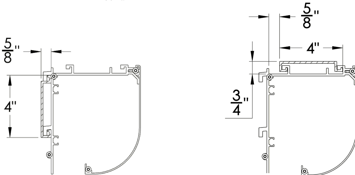
Figure 4: (From left) Basic dimensions shown of wall mount with frame rails. Basic dimensions shown of ceiling mount with frame rails.
